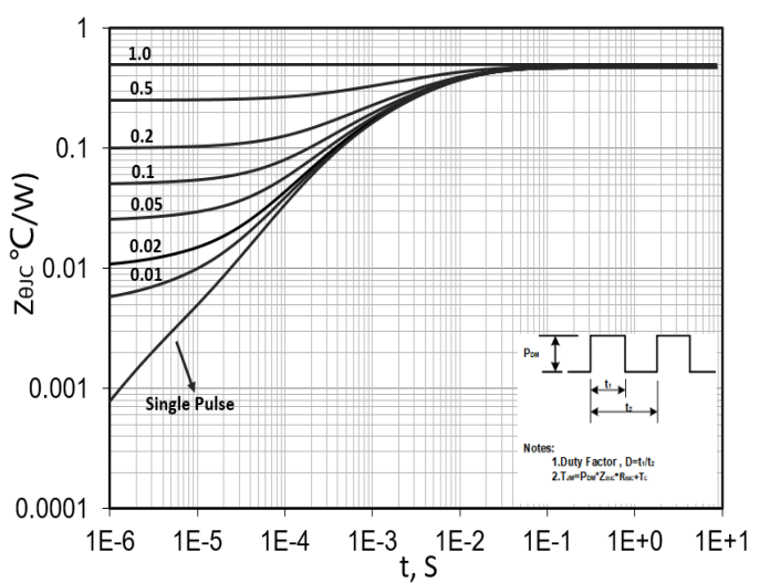
Figure 12. Transient Thermal Response Curve (TO-220)
