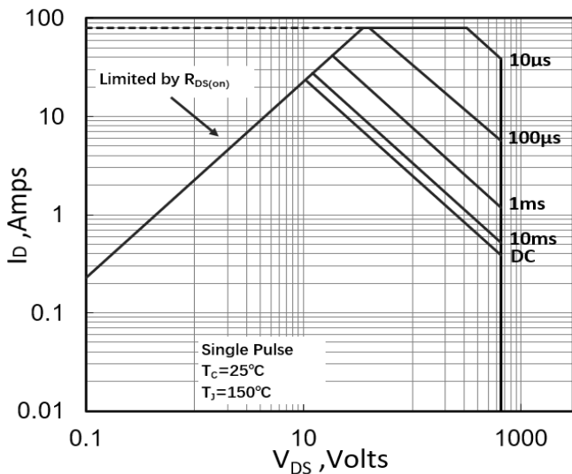
Figure 11. Maximum Safe Operating Area (TO-220)
